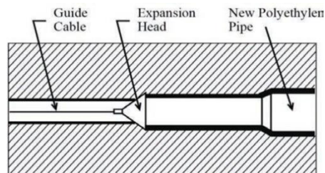
Figure 2. 7: Pipe bursting process
